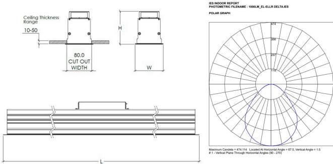
NORMALISED POLAR CURVE
